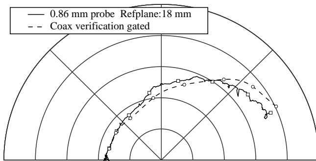
Fig. 16. Reflection coefficient measured from 0.1 to 40 GHz with the 0.85 mm probe and coaxially. Markers every 5 GHz.
